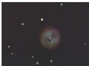
M97
